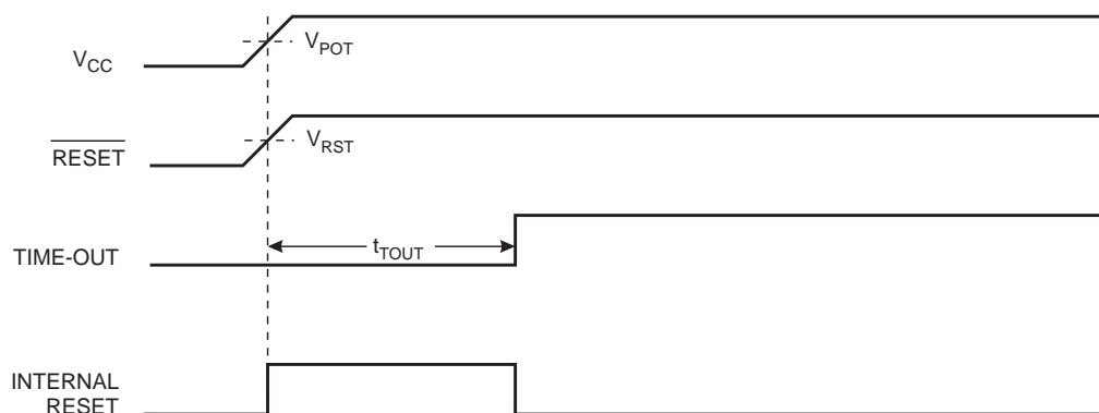
Figure 22. MCU Start-up, \overline{\text{RESET}} Tied to V_{CC} .
